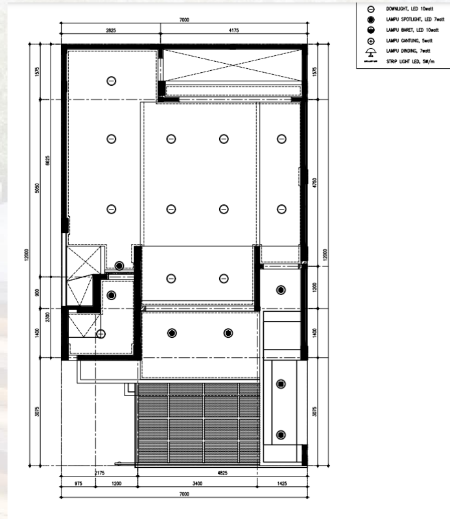
Lantai 1
